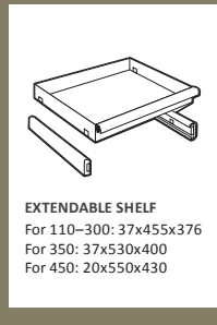
REMOVABLE SHELF* For 60: 20x375x350 For 110-300: 20x475x376 For 350: 20x550x400 For 360: 20x710x542 For 450: 20x550x430
